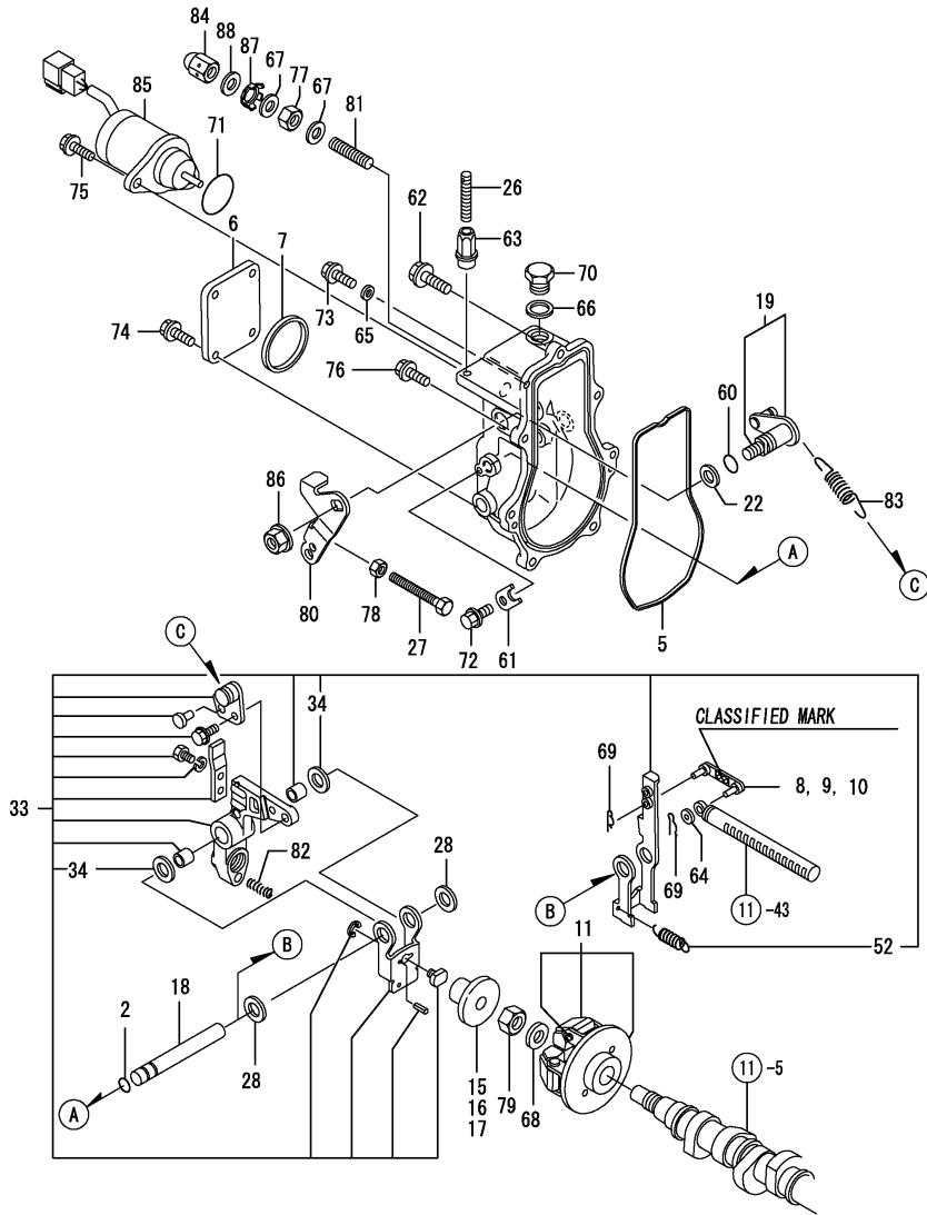
Fig.12. GOVERNOR
