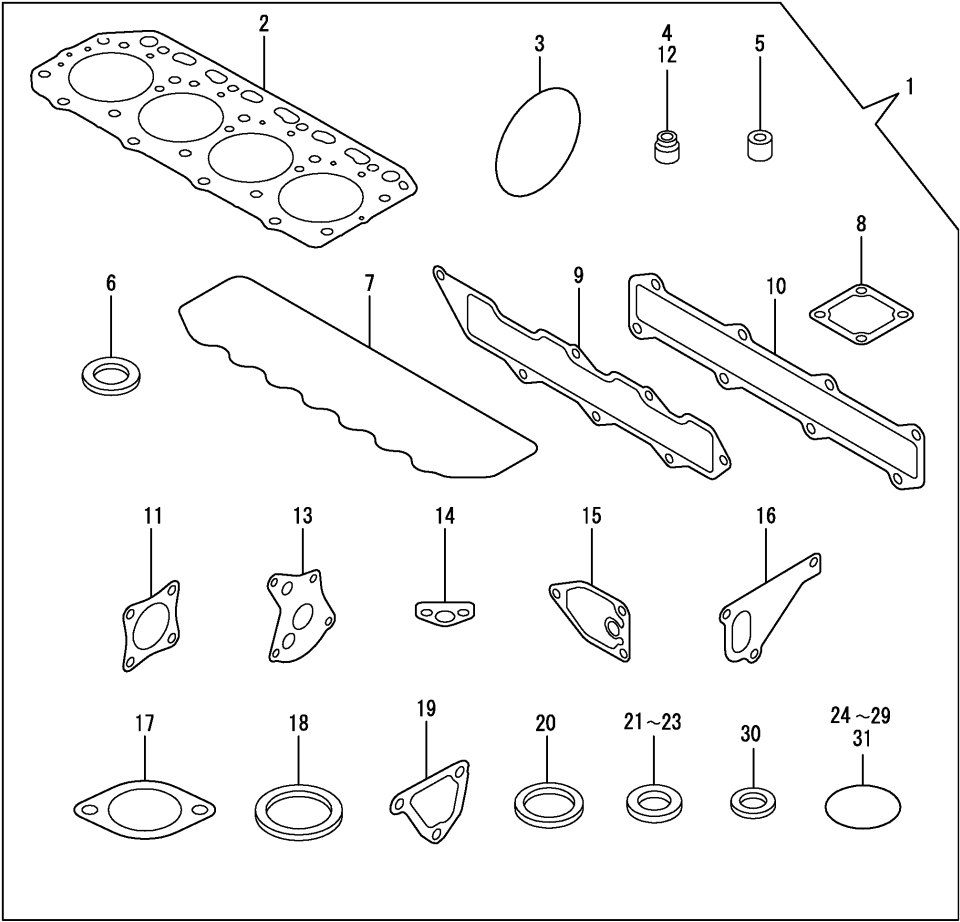
Fig.17. GASKET SET
