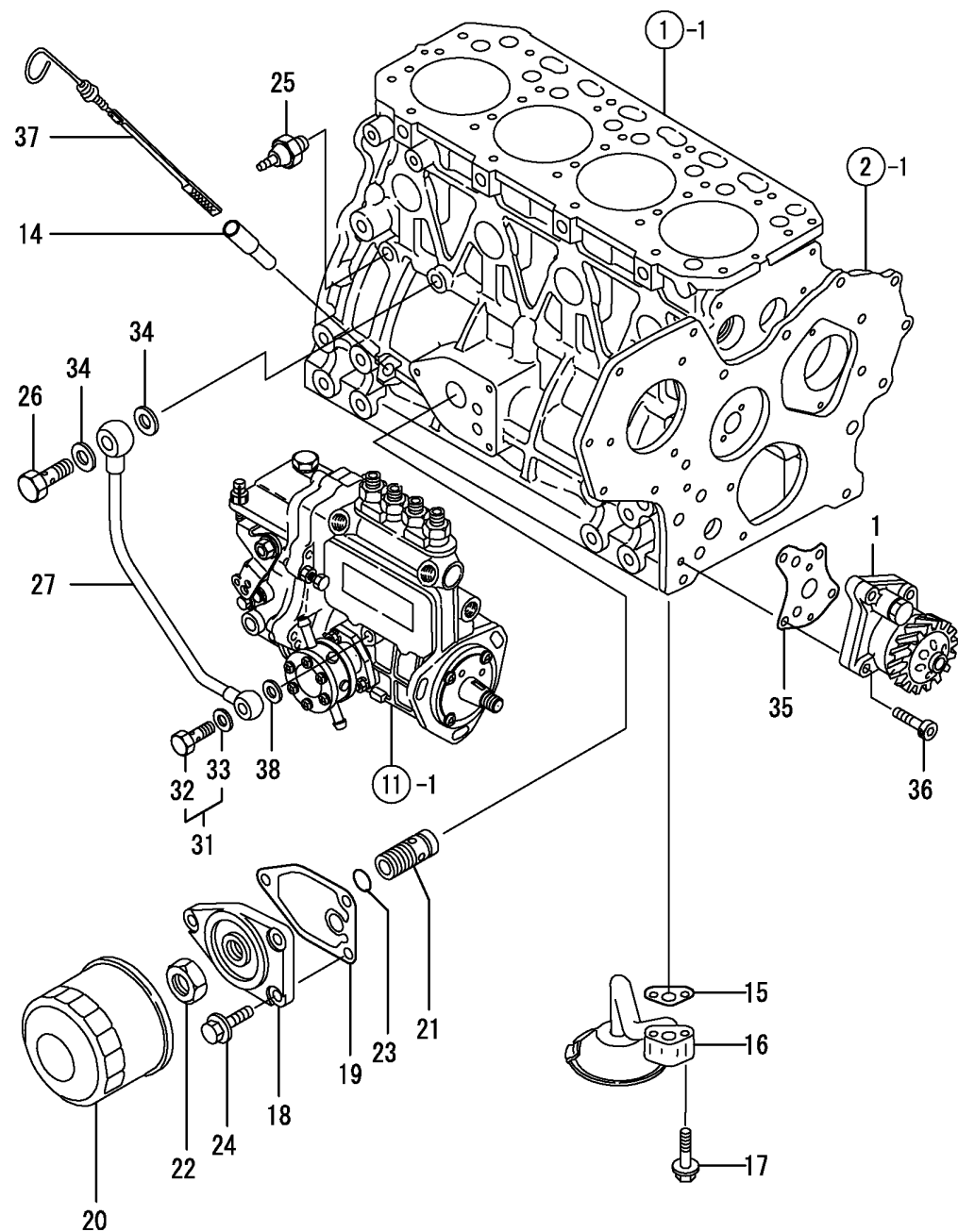
Fig.9. LUB.OIL SYSTEM
