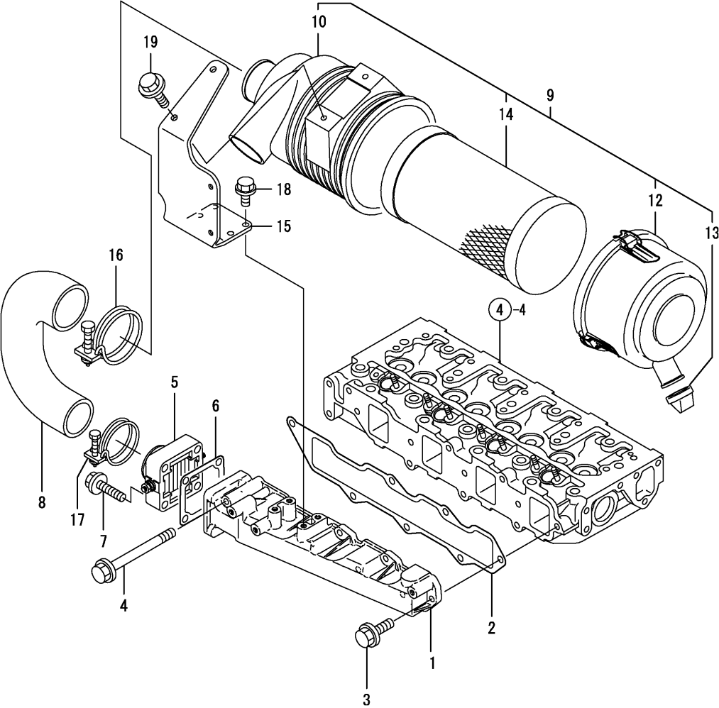
Fig.5. SUCTION MANIFOLD & AIR CLEANER
