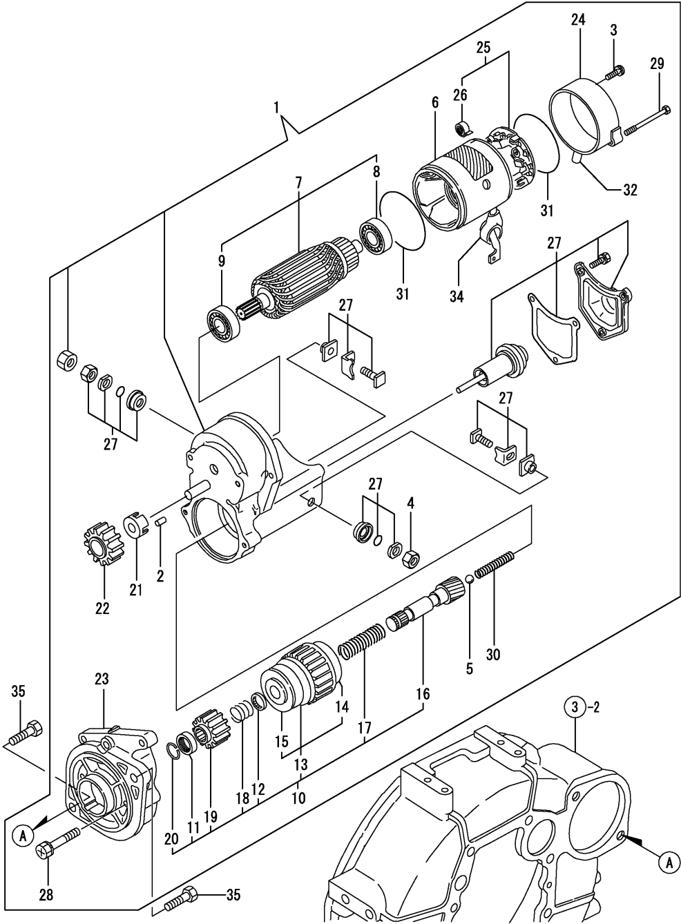
Fig.15. STARTING MOTOR
