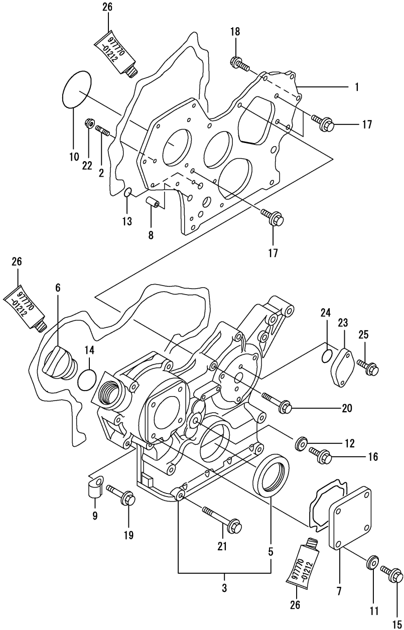
Fig.2. GEAR HOUSING
