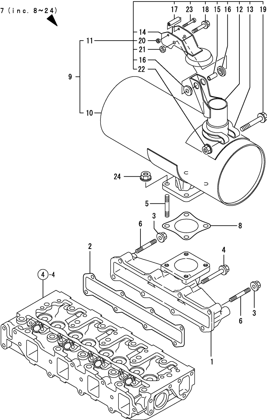
Fig.6. EXHAUST MANIFOLD & SILENCER
