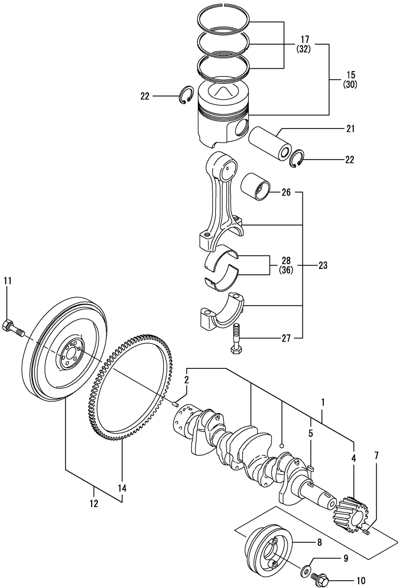
Fig.8. CRANKSHAFT & PISTON
